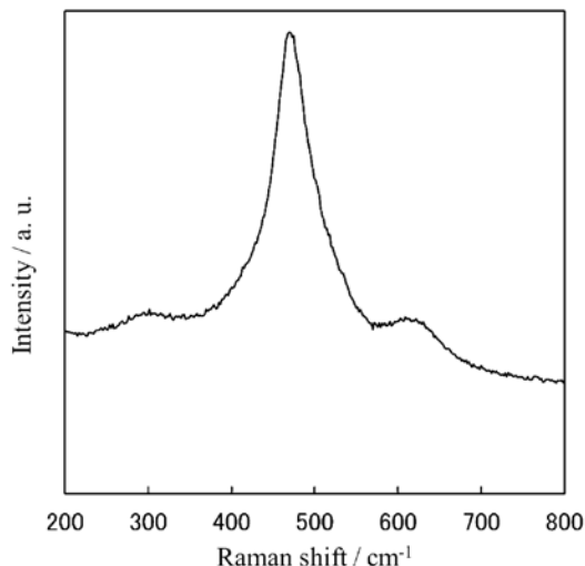
Fig.2 Raman spectrum of 1.0wt.%Cu/ Ce_{0.7}Zr_{0.3}O_2 .
