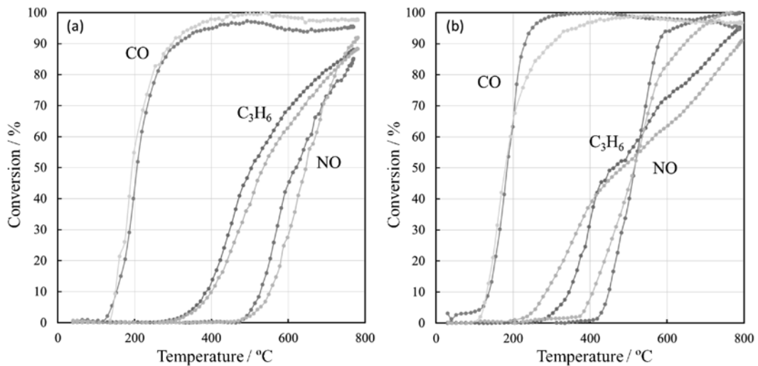
Fig.5 Conversion of CO, C 3 H 6 , and NO over (a) cordierite and (b) SiC honeycomb catalysts compared with 1.0wt.%Cu/Ce 0.7 Zr 0.3 O 2 (light-colored line).
