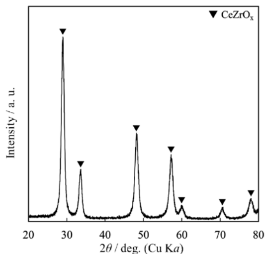
Fig.1 XRD pattern of 1.0wt.%Cu/ Ce_{0.7}Zr_{0.3}O_2 .
