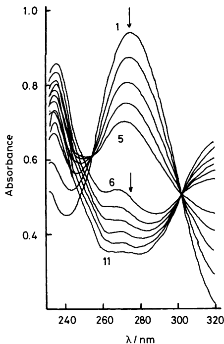
Figure 1. Spectral time study for the reaction of (IIIa) with (Ia) in the presence of CTAB at pH 7.30, 0.02M-phosphate buffer (0.4M-KCl), and 10 °C. [(IIIa)] 1.6 \times 10^{-4} M, [(Ia)] 1.00 \times 10^{-3} M, [CTAB] 1.00 \times 10^{-2} M. Spectra curves 1–5 and 6–11 show repeated scans and scans after a 10 min interval, at 480 nm \text{min}^{-1} , respectively
