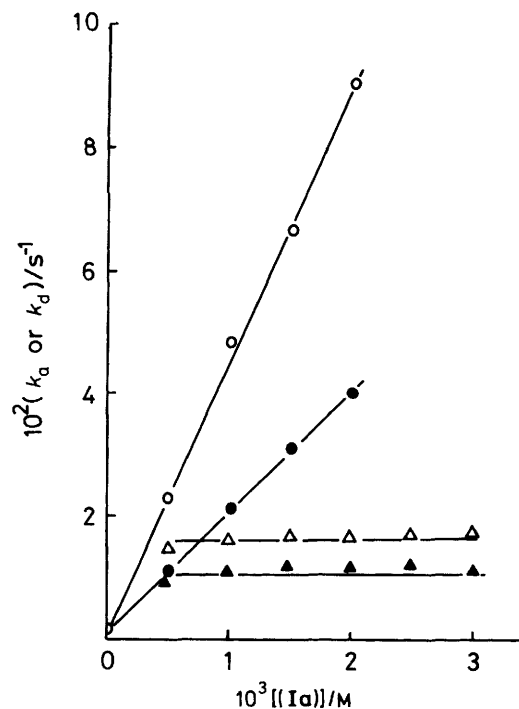
Figure 3. Effect of catalyst ( Ia ) concentration on the rate in the presence of CTAB at pH 7.30, 0.02M-phosphate buffer, and 25 °C. [( IIIa )] 1.0 \times 10^{-4} M, [CTAB] 3.00 \times 10^{-2} M, (●, ○) acylation rate constants, ● with D-( IIIa ), ○ with L-( IIIa ); (▲, △) deacylation rate constants, ▲ with D-( IIIa ), △ with L-( IIIa )
