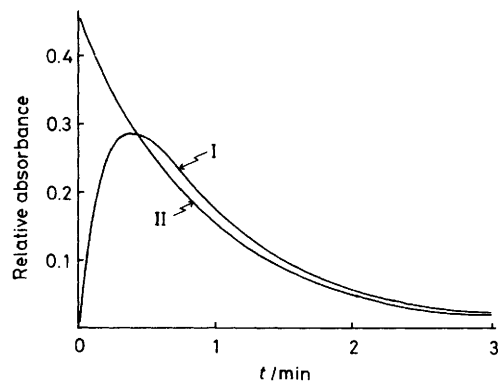
Figure 2. Relative absorbances during the reaction of (IIIa) with (Ia) in the presence of CTAB (curve I, at 245 nm; curve II, at 255 nm). Conditions; pH 7.30, 0.02M-phosphate buffer, and 25 °C. [(IIIa)] 1.6 \times 10^{-4} M, [(Ia)] 1.00 \times 10^{-3} M, [CTAB] 1.00 \times 10^{-2} M
