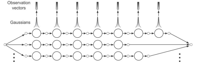
Figure 20: Huge HMM network representing units. Every unique path represents exactly one unit.
