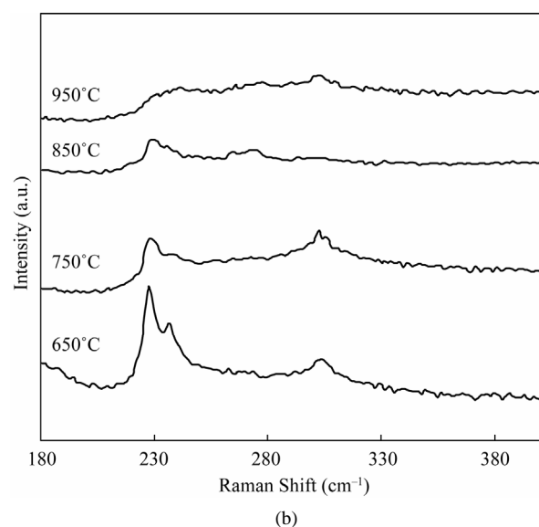
Figure 7. (a) Raman spectra of the samples synthesized at 650°C, 750°C, 850°C and 950°C in high frequency region; (b) Raman spectra of the samples synthesized at 650°C, 750°C, 850°C and 950°C in low frequency region.
