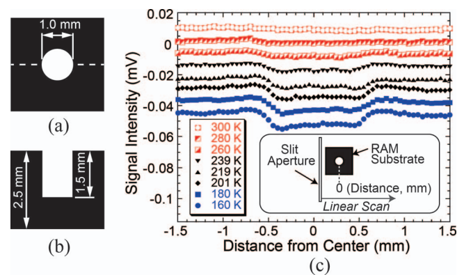
FIG. 2. (a) Schematic diagram of the sample. (b) Cross-sectional drawing of the sample along the dotted line in (a). (c) One-dimensional scans of the sample at various sample temperatures from 300 K to 160 K. The inset in (c) shows the scanning arrangement. The sample is 30 mm in diameter. In (a) and (b), only the area corresponding to the field of view (3 mm \times 3 mm) in the imaging experiment (Fig. 3) is depicted.
