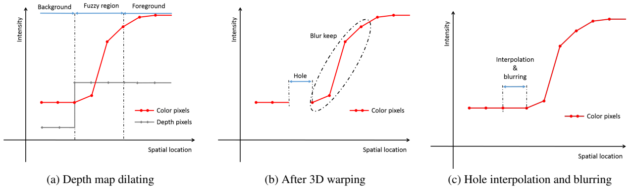
Figure 2. Color image and depth map conditions of each process.
