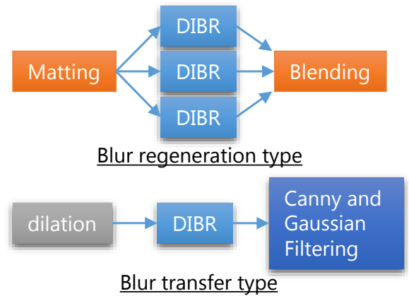
Figure 3. Two types of view synthesis for boundary treatment.
