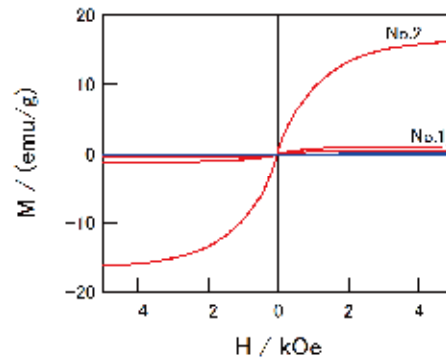
Fig. 6a Magnetization curves of the several pieces of the old seto black pottery.
